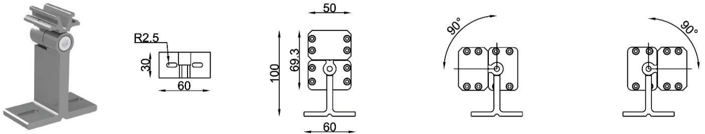
ARK-MB Adjustable mounting option for applications that require angle adjustments. Rotatable up to 180 Degrees.
