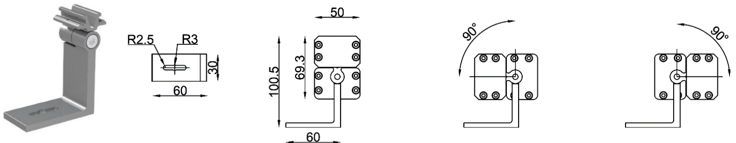
ARK-ML L-shape adjustable mounting option for applications that require angle adjustments. Rotatable up to 180 Degrees.
