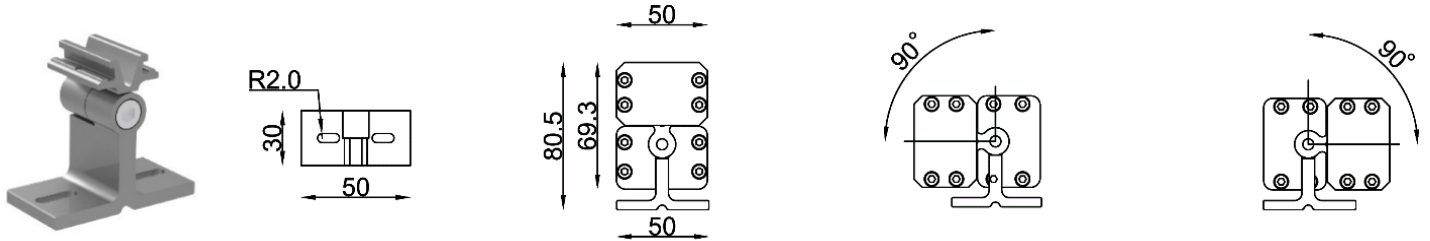
ARK-MA Adjustable mounting option for applications that require angle adjustments. Rotatable up to 180 Degrees.
