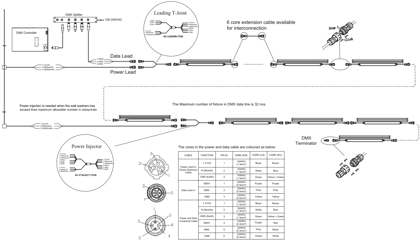
Maximum power and number of 4-ft fixtures can be clustered in a daisy chain:
