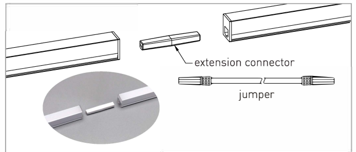
Step 2: Splicing multiple products by extension connector or jumper.
