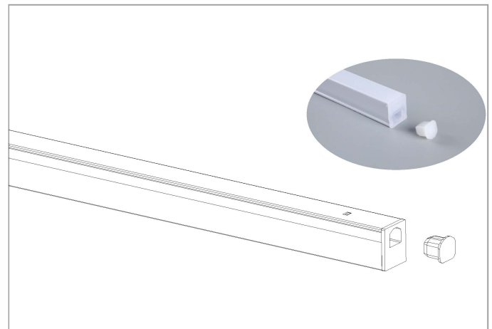
Step 4: Seal the terminal socket by inserting the rubber end cap, which is required for the product at the tail in the same string.
